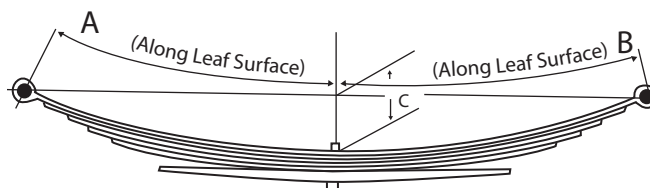
TYPE B (Two Stage Spring)
